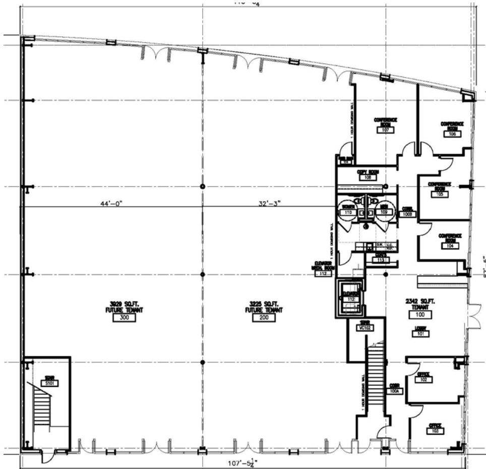
1st Floor
